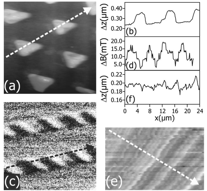
FIG. 3. (a) AFM image of an hexagonal array of Au triangles [image size (IS) \sim 20 \mu\text{m} \times 20 \mu\text{m} , grayscale spans (GS) \sim 100 nm]. (b) Linescan in the direction indicated in (a). (c) Magnetic image of a magnetic imaging reference sample (MIRS) (IS \sim 20 \mu\text{m} \times 18 \mu\text{m} , GS \sim 18 mT). (d) Linescan of (c) in direction indicated. (e) Topographic image of MIRS (IS \sim 20 \mu\text{m} \times 12 \mu\text{m} , GS \sim 100 nm). (f) Linescan in direction indicated in (e).
