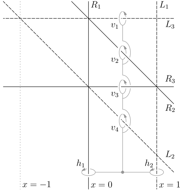
FIGURE 1. The divisor V := L + R \subset \Phi
