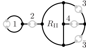
FIGURE 5. A type D_5 singular point: irreducible curves
