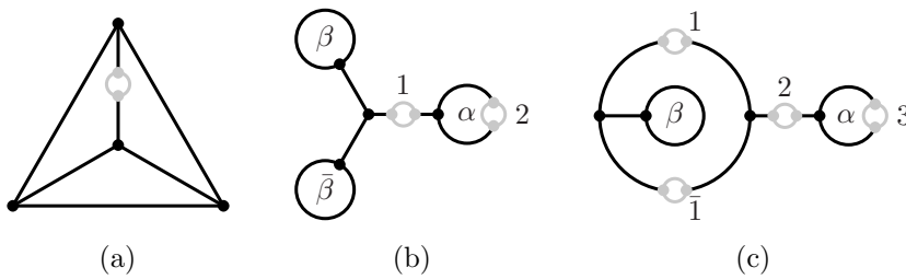
FIGURE 4. A type \mathbf{D}_p singular point, p \geq 7
