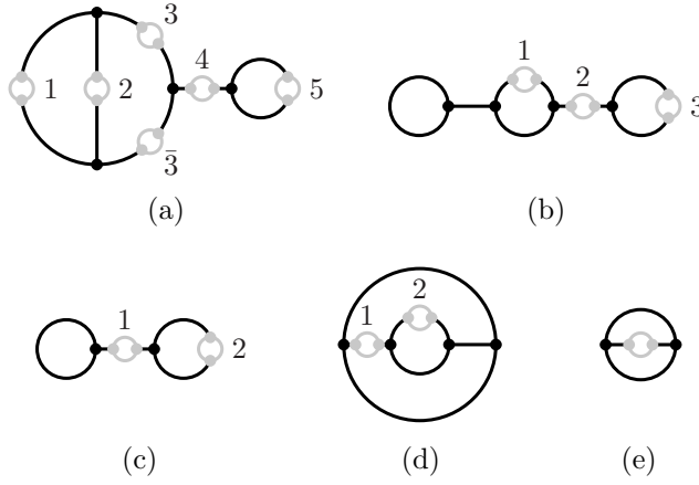
FIGURE 7. A type D_p singular point, p \geq 7 : reducible curves
