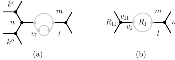
FIGURE 8. Regions used in the computation
