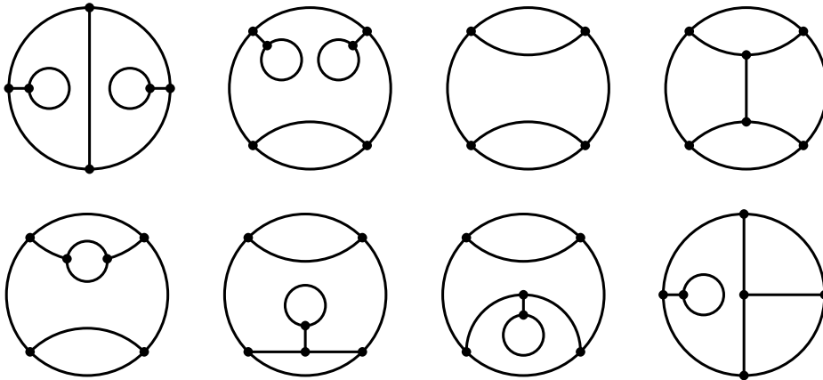
FIGURE 6. A type D_5 singular point: all curves
