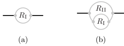
FIGURE 3. A bigonal (a) and bibigonal (b) insertions
