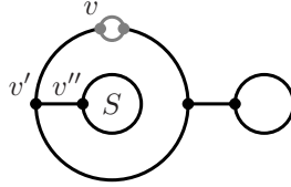
FIGURE 8. The set of singularities \mathbf{E}_7 \oplus 2\mathbf{A}_6
