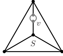
FIGURE 9. The set of singularities \mathbf{E}_7 \oplus 2\mathbf{A}_4 \oplus 2\mathbf{A}_2
