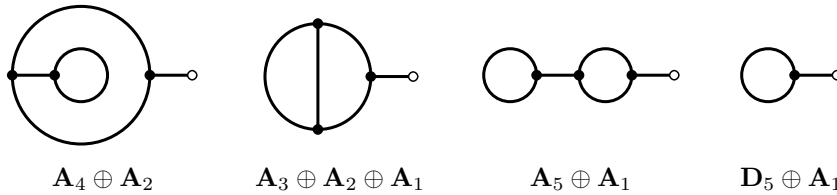
fig.pert FIGURE 11. Perturbations of \mathbf{E}_7 with nonabelian fundamental group
