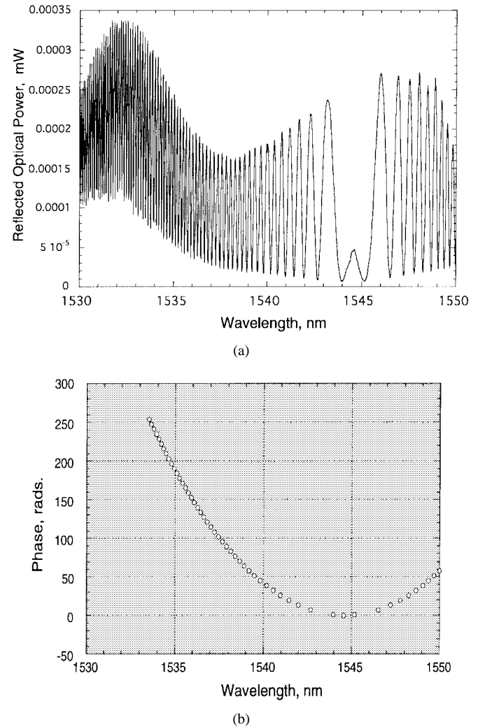
Fig. 20. Interferometer phase response (a) direct spectral output and (b) phase versus wavelength.
