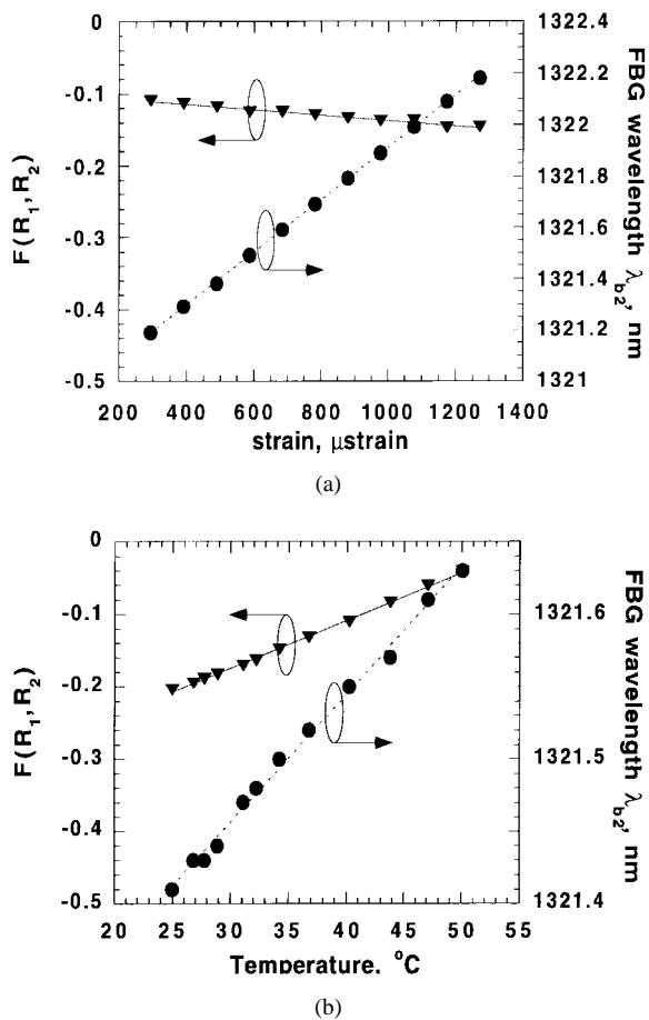
Fig. 24. (a) F(R_1, R_2) and \lambda_{b2} versus strain in \mu\text{strain} , measured while the sensor was held at a temperature of 38^{\circ}\text{C} , and linear fits to the data. (b) F(R_1, R_2) and \lambda_{b2} versus temperature in ^{\circ}\text{C} , measured while the sensor was held at 590 \mu\text{strain} applied, and linear fits to the data.
