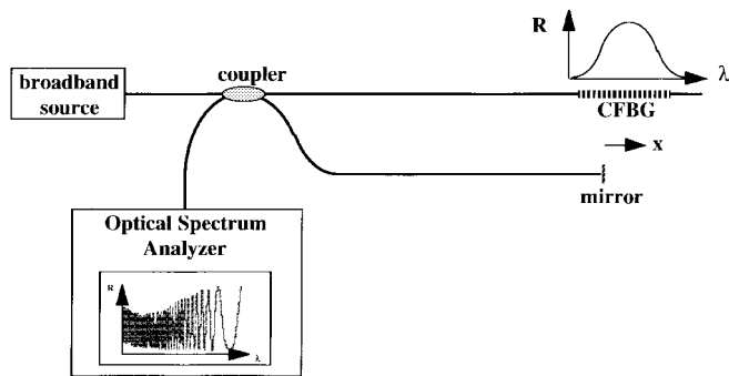
Fig. 19. Chirped grating fiber Michelson interferometer.
