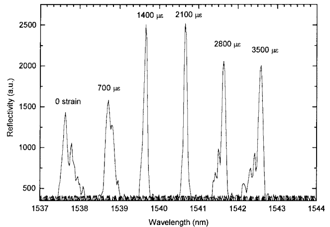
Fig. 13. Reflectance spectra of chirped grating tapered from 115 to 105 \mu\text{m} before grating under \sim 1700 \mu\text{E} and measured under different strains.
