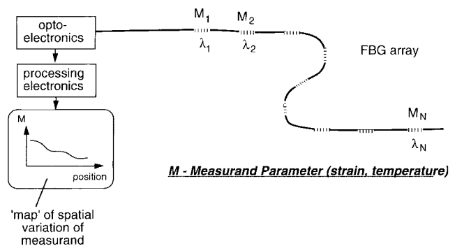
Fig. 2. Quasi-distributed sensor system using FBG elements.
