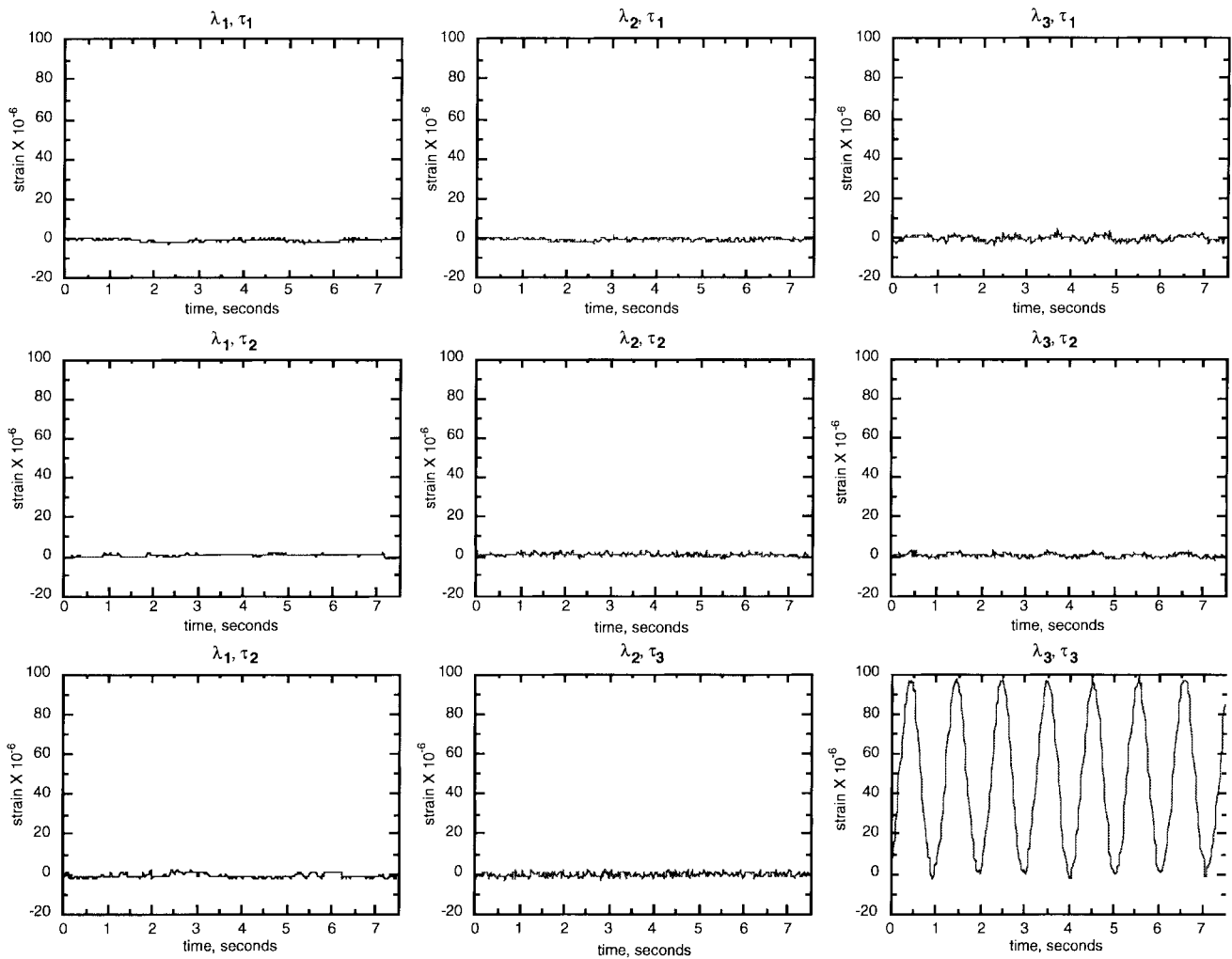
Fig. 10. WDM/TDM system outputs for a 3 × 3 array.
