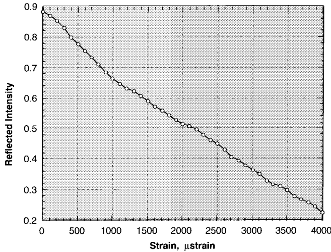
Fig. 16. Change in reflectivity of the asymmetric FBG at a fixed “probe” wavelength of 1534 nm.
