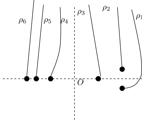
FIGURE 2. Generators in the fiber y = -\varepsilon
