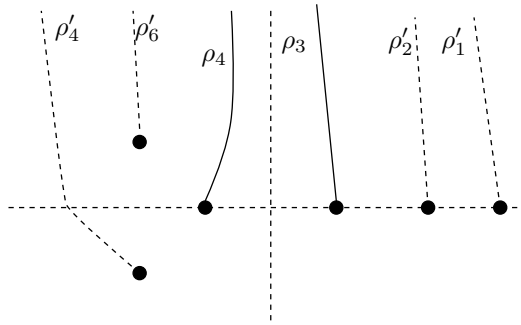
FIGURE 3. Generators in the fiber y = \varepsilon
