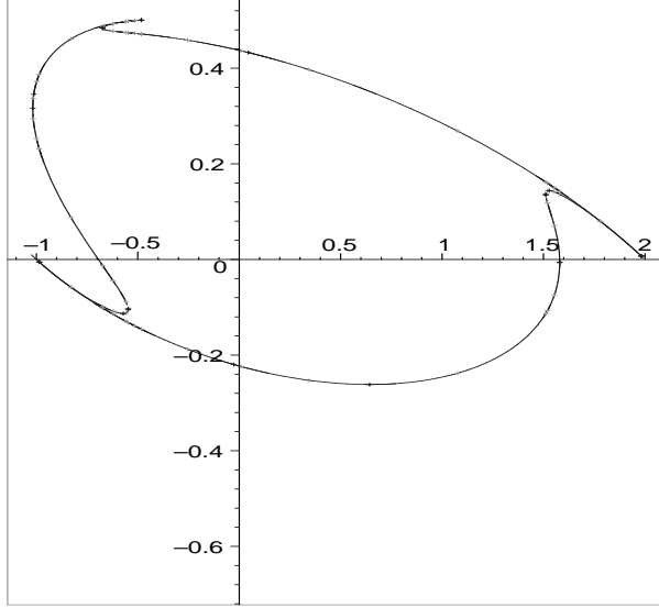
FIGURE 1. The graph of B
