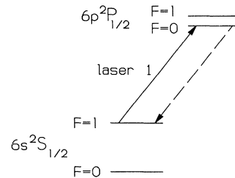
FIG. 5. Energy levels of ^{199}\text{Hg}^+ . The transition between the 2S_{1/2} and 2P_{1/2} states is at 194 nm. The hyperfine splittings in the 2S_{1/2} and 2P_{1/2} states are 40.5 and 6.9 GHz, respectively. The 2S_{1/2} ( F = 1 ) state is detected by exciting the 2S_{1/2} ( F = 1 ) \rightarrow 2P_{1/2} ( F = 0 ) transition with laser 1.
