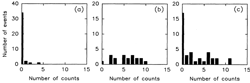
FIG. 9. Photon count distributions for a single ^{199}\text{Hg}^+ ion prepared in (a) the ( F=0 , M_F=0 ) state, (b) the ( F=1 , M_F=0 ) state, and (c) an equal superposition of these two states. The bars represent the number of cases in which a given number of fluorescence photons was detected when the detection laser was applied. The number of measurements was 38 for (a), 19 for (b), and 38 for (c).
